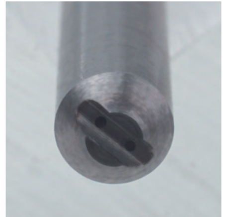
Shank end suitable for minimal quantity lubrication without build-up or dead pockets of coolant.
