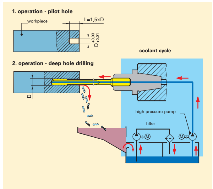
Fig. 5: Deep hole drilling on conventional machine tools
